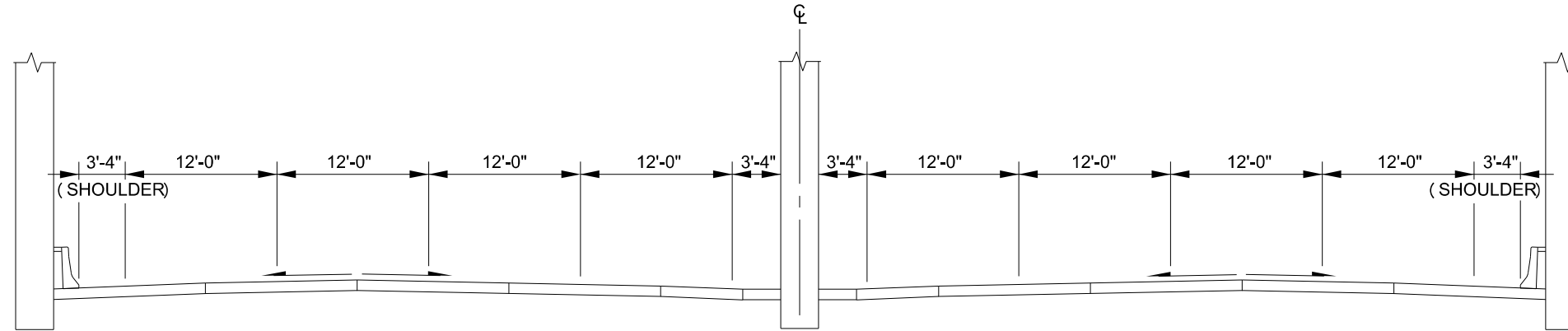
WEST DODGE ROAD RECOMMENDED CONCEPT PROPOSED CONDITIONS WEST DODGE BRIDGE UNDERPASS AT 156TH, 168TH AND 180TH ST
