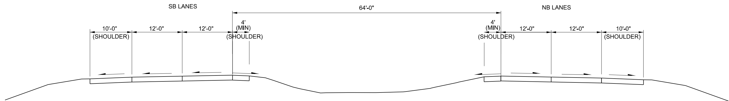
US 75 EXISTING CONDITIONS BETWEEN N-370 AND CORNHUSKER
