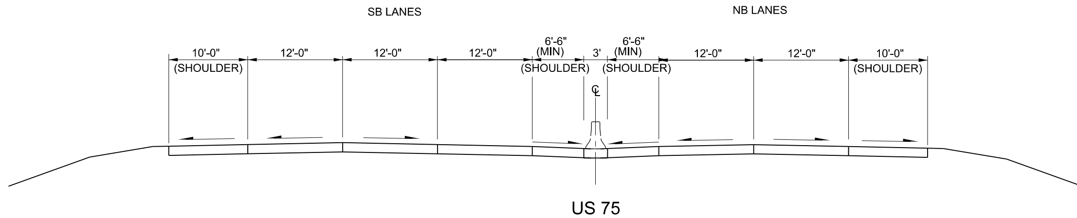
US 75 EXISTING CONDITIONS BETWEEN CHANDLER RD AND Q ST
