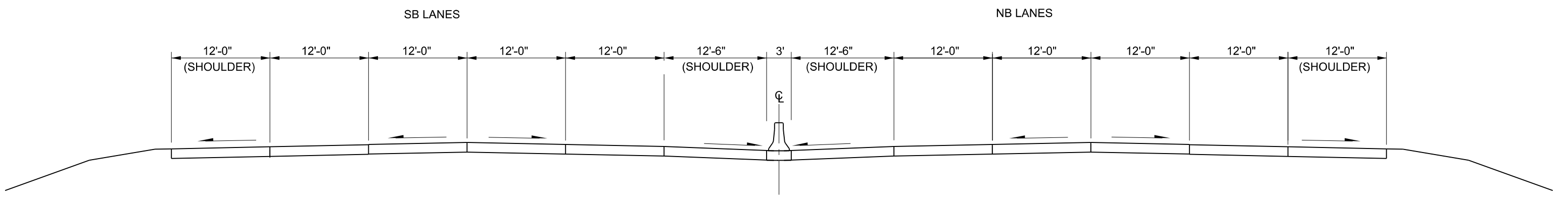
US 75 RECOMMENDED CONCEPT PROPOSED CONDITIONS BETWEEN CHANDLER RD AND Q ST
