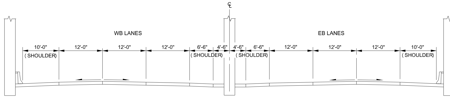
WEST DODGE ROAD EXISTING CONDITIONS WEST DODGE BRIDGE UNDERPASS AT 156TH ST, 168TH AND 180TH ST
