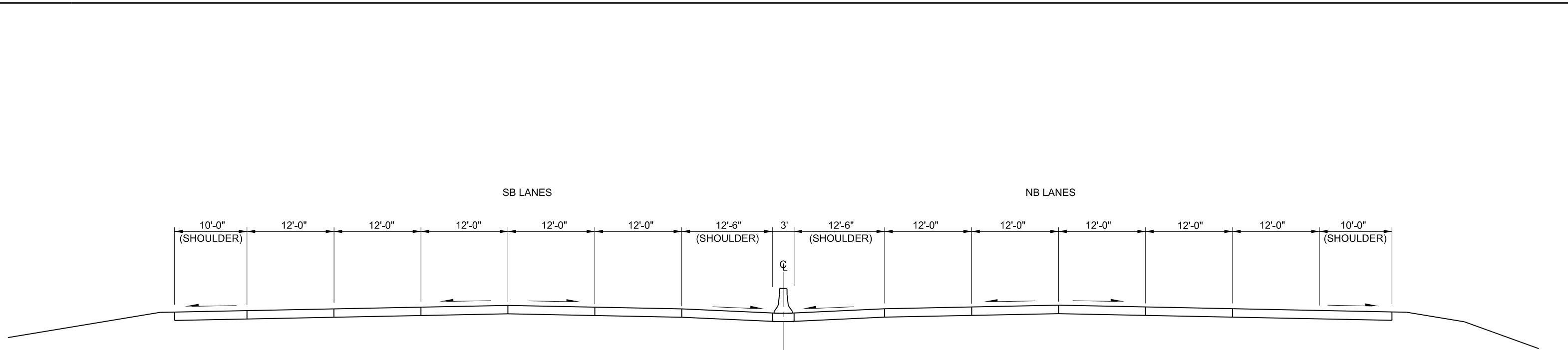
I-680 EXISTING CONDITIONS BETWEEN WEST CENTER RD AND PACIFIC ST
