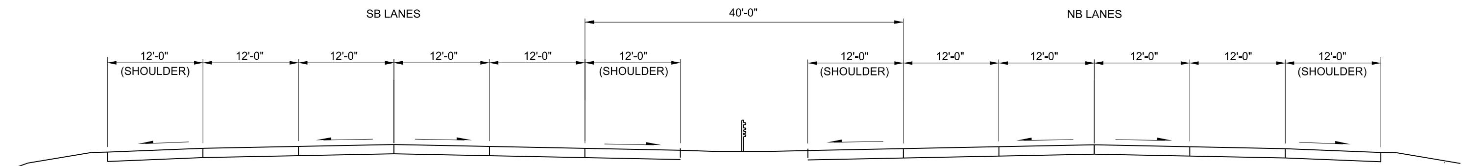
US 75 RECOMMENDED CONCEPT PROPOSED CONDITIONS BETWEEN N-370 AND CORNHUSKER
