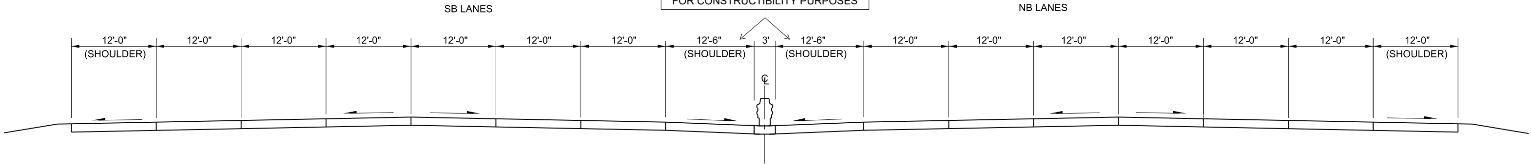
I-680 RECOMMENDED CONCEPT PROPOSED CONDITIONS BETWEEN WEST CENTER RD AND PACIFIC ST
