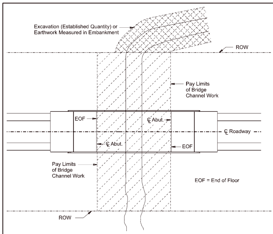
Exhibit 13.3 Pay Limits for Bridge Channel Work
