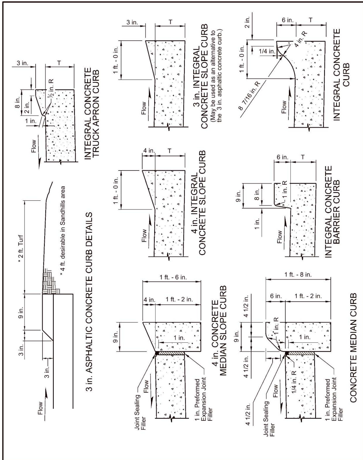
Exhibit 6.12 Typical Curb Details
