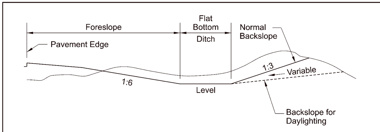
Exhibit 6.17 Daylighting
