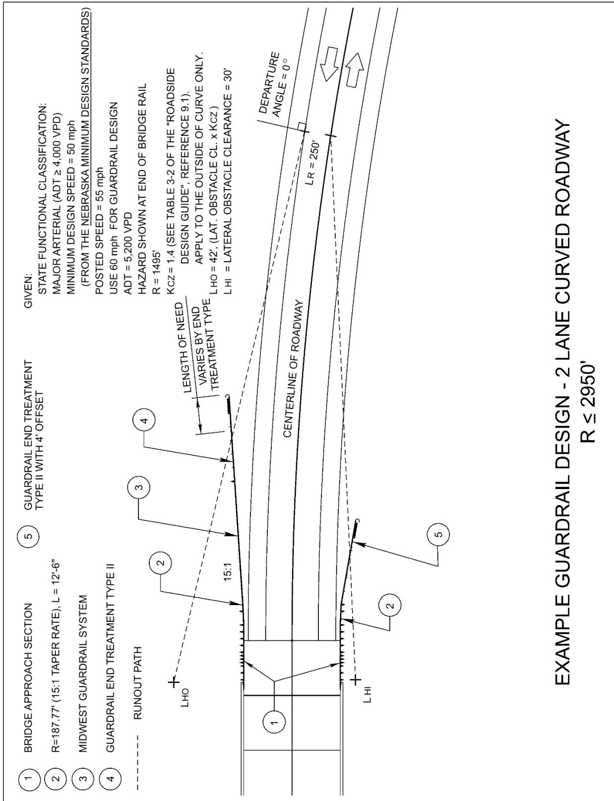
Exhibit 9.12 Example Guardrail Design at a Bridge: 2-Lane, 2-Way Curved Roadway; R ≤ 2950'
